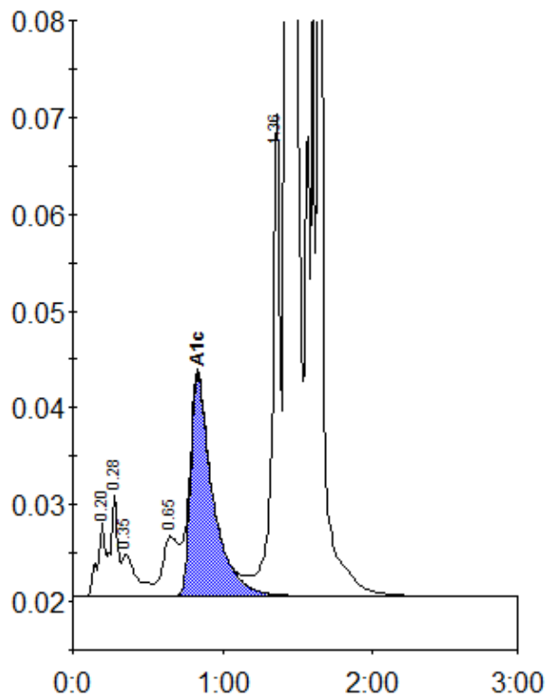
Peak table - ID: 10427407
